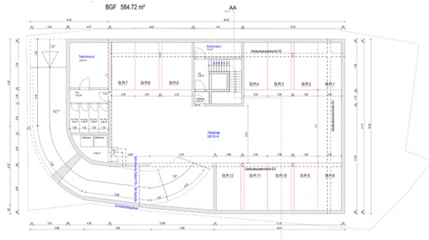
underground car park
